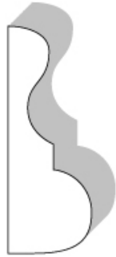
Chair Rail #260 7/8" X 2 3/8"
