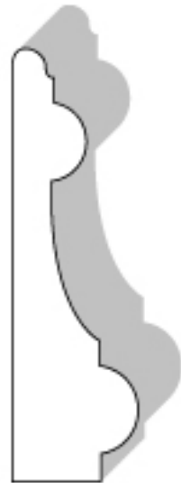
Chair Rail #128 3/4" X 2 1/2"
