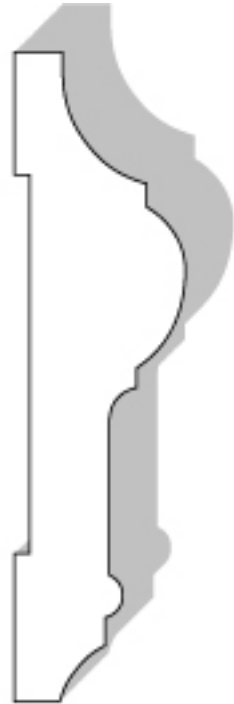
Chair Rail #156 3/4" X 3 3/8"
