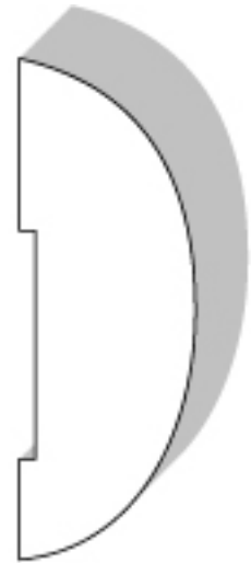
Chair Rail #157 13/16" X 2 3/8"
