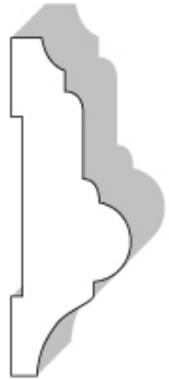
Chair Rail #137 3/4" X 2 1/2"
