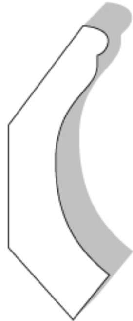
Crown Mould #218 1 3/16" X 3 1/8"
