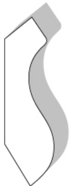
Crown Mould #226 3/4" X 2 7/8"
