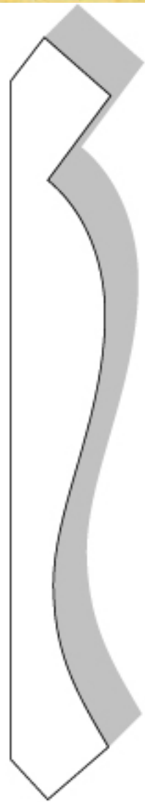
Crown Mould #139 3/4" X 5 3/4"
