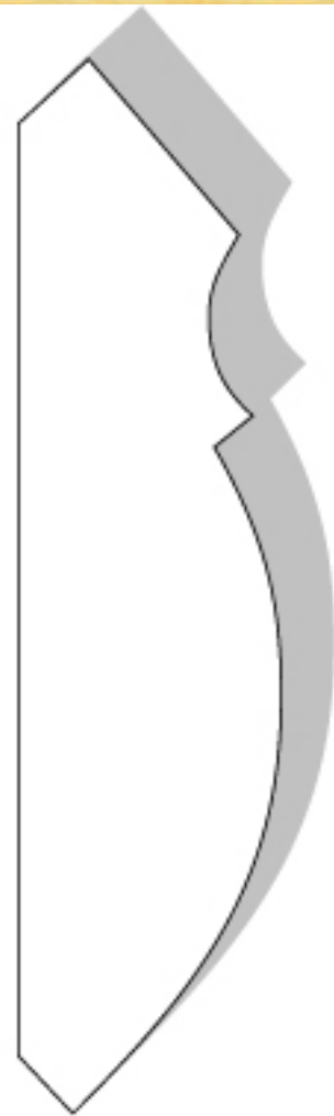
Crown Mould #245 1 1/4" X 5"
