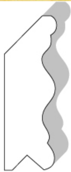
Crown Mould #230 7/8" X 2 3/4"
