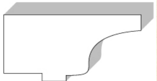
Header Mould #233 1 3/16" x 2 3/4"
