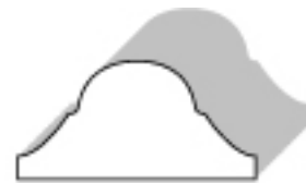
Panel Mould #154 9/16" X 1 1/8"
