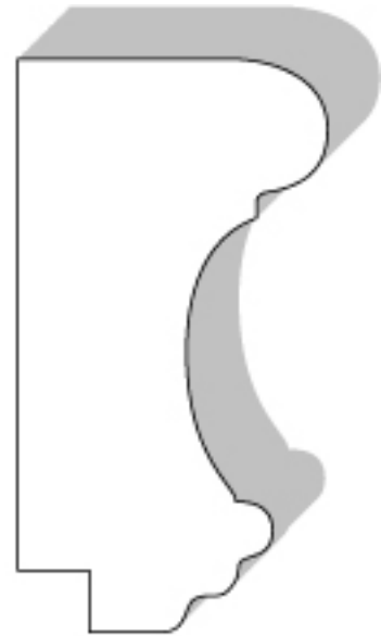
Wainscap #162 1 1/2" X 2 3/4"
