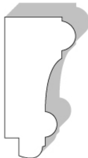
Wainscap #129 1 1/4" X 2 1/2"
